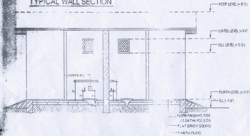
TOILET BLOCK SECTION AT C-C TYPE - SMALL SCHOOL BASIC (SS-B)
