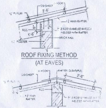
ROOF FIXING METHOD
