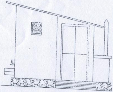
SIDE ELEVATION TYPE - SMALL SCHOOL BASIC (SS-B)
