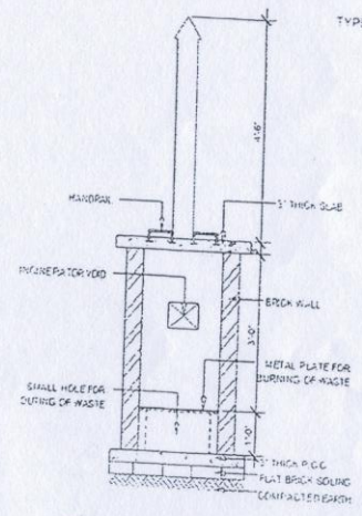
TYPICAL INCINERATOR SECTION AT C-C
