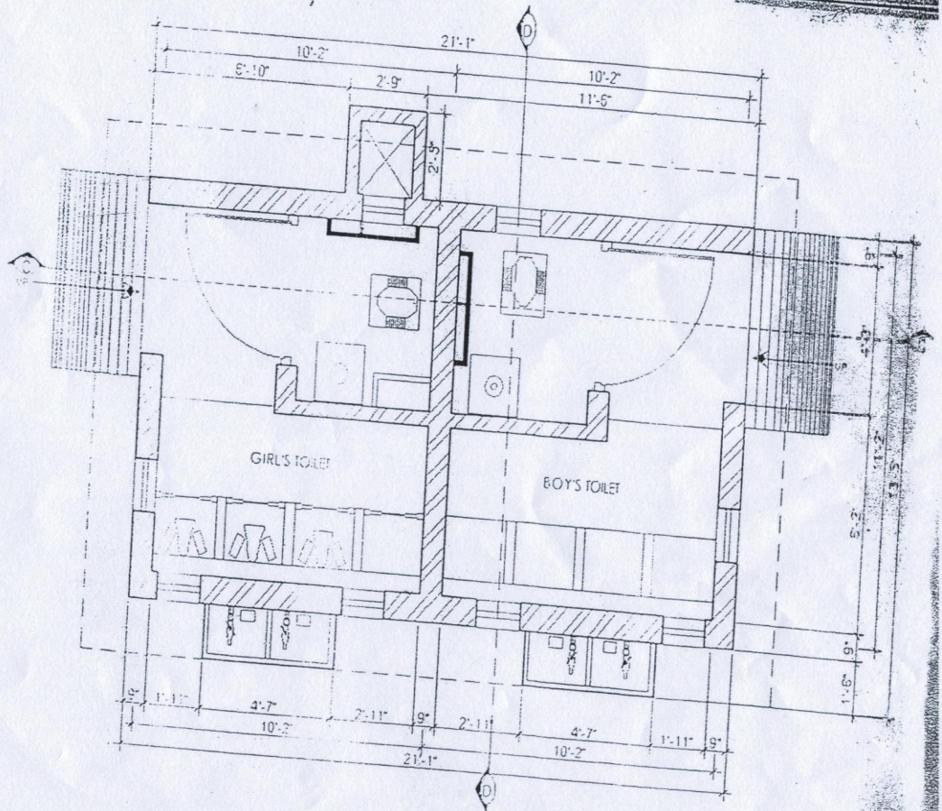
TYPE SMALL SCHOOL BASIC(SS - B) TOILET BLOCK PLAN DIM IN FT AND INCH
