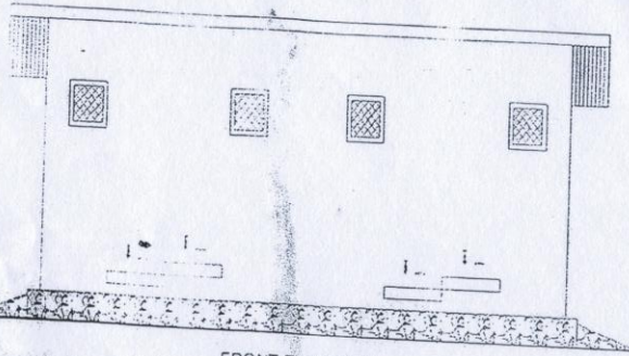
FRONT ELEVATION TYPE - SMALL SCHOOL BASIC (SS-B)
