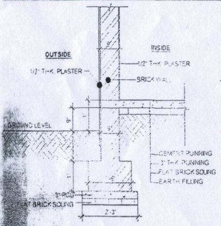
TYPICAL WALL SECTION
